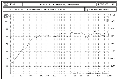
Frequency response,SPL/2.83v
