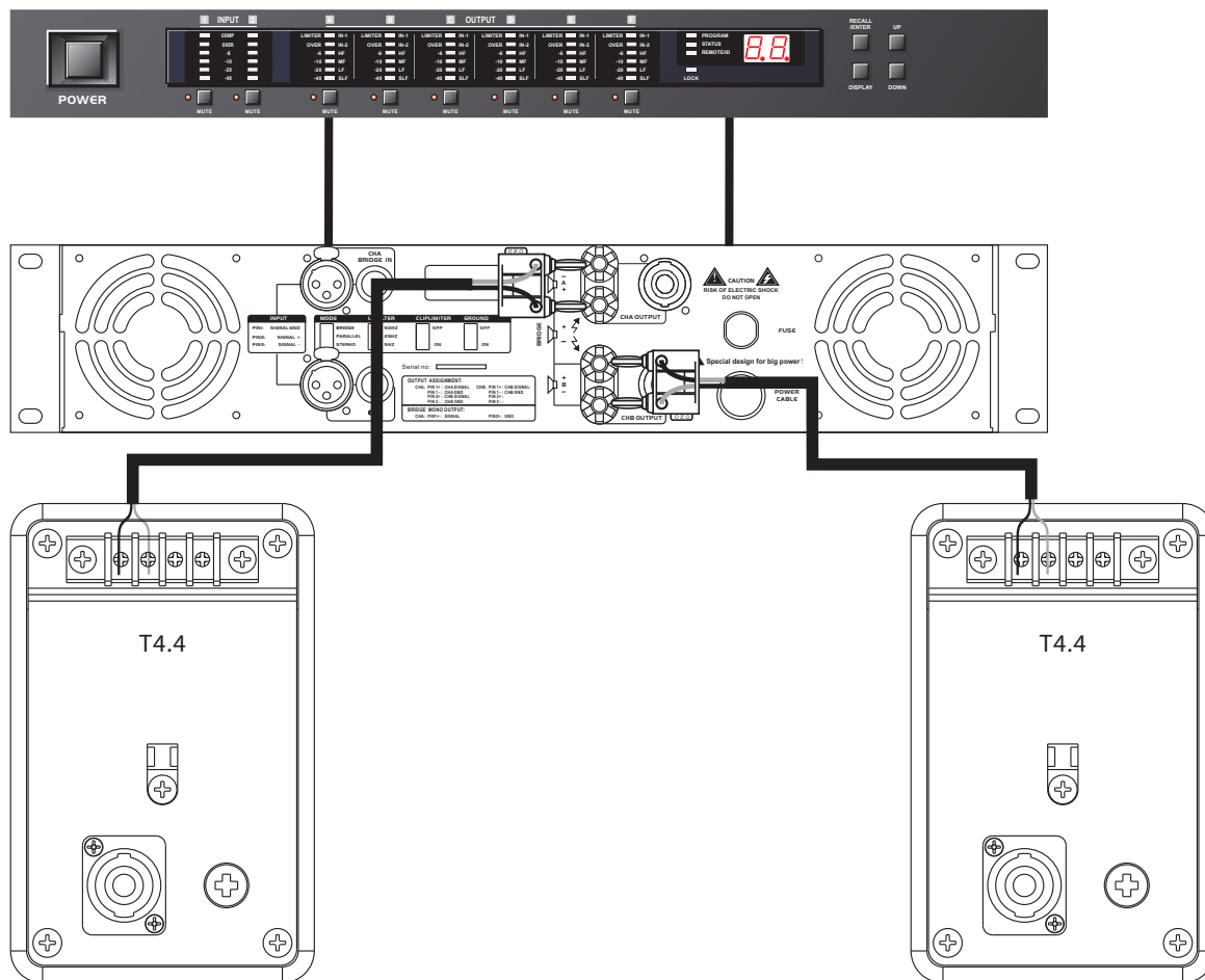
Processor (Optional EQ curves available on CD)
